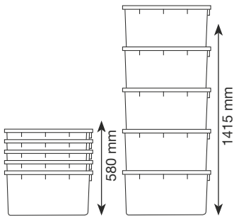
5 Tau 50 stacked pieces = 1415 mm inserted pieces = 580 mm
