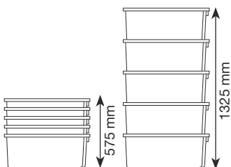
5 Tau 70 stacked pieces = 1325 mm inserted pieces = 575 mm
